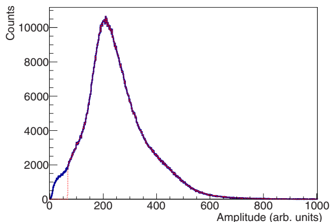
FIG. 2. The FF amplitude distribution from the pulse shape analysis of the ^{237}\text{Np} target. The blue curve corresponds to the analysis without additional threshold for the exclusion of low amplitude pulses, and the red dotted line corresponds to the amplitude distribution with the threshold chosen as discussed in Sec. III A.
