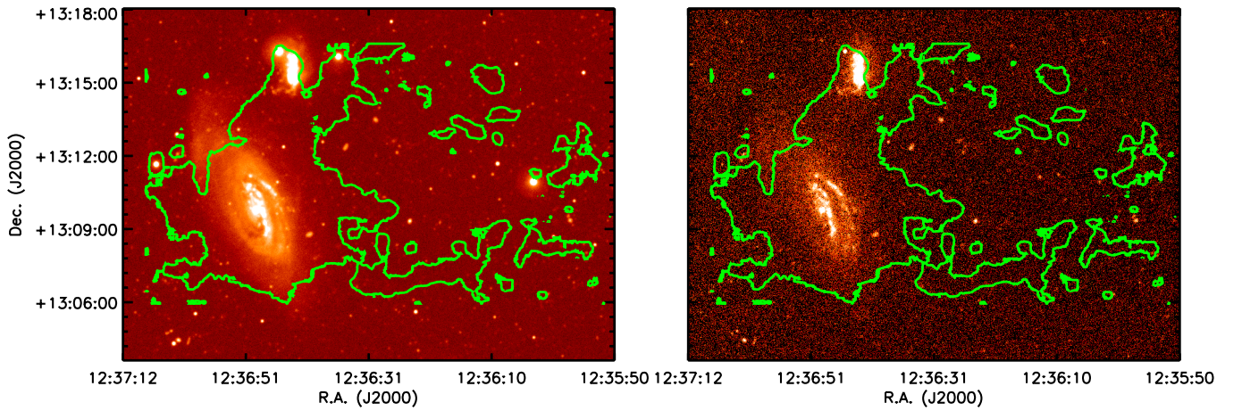
Fig. 9. GALEX NUV ( left ) and FUV ( right ) images of NGC 4569 with contour levels showing the H\alpha+[NII] surface-brightness level of 10^{-18} \text{ erg s}^{-1} \text{ cm}^{-2} \text{ arcsec}^{-2} .
