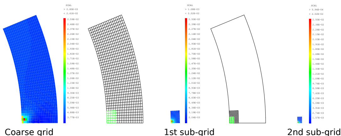
FIGURE 6 – Exemple for the 2D( r,\theta ) test case · Coarse mesh size : 54.5 \mu\text{m} \cdot \beta = 1\%
