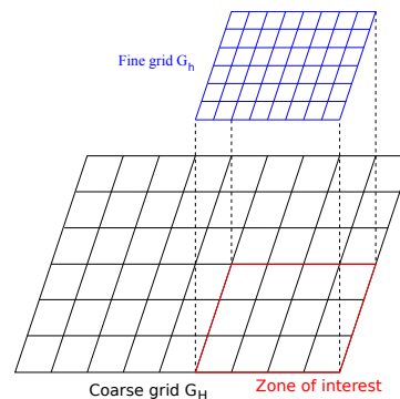
FIGURE 2 – Example of hierarchical meshes used in LDC method
