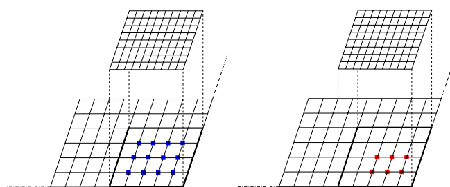
FIGURE 4 – Example of restriction zone A_H (on the left) and correction zone (on the right) in the case of a 5-point stencil operator for hierarchical meshes
