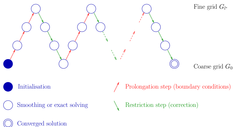
FIGURE 1 – Representation of the iterative process in \wedge -cycle
