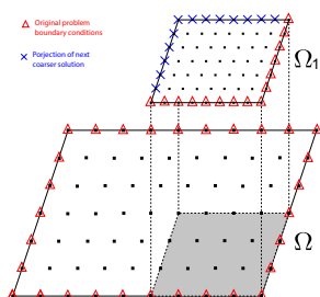
FIGURE 3 – Example of boundary conditions on G_h for hierarchical meshes
