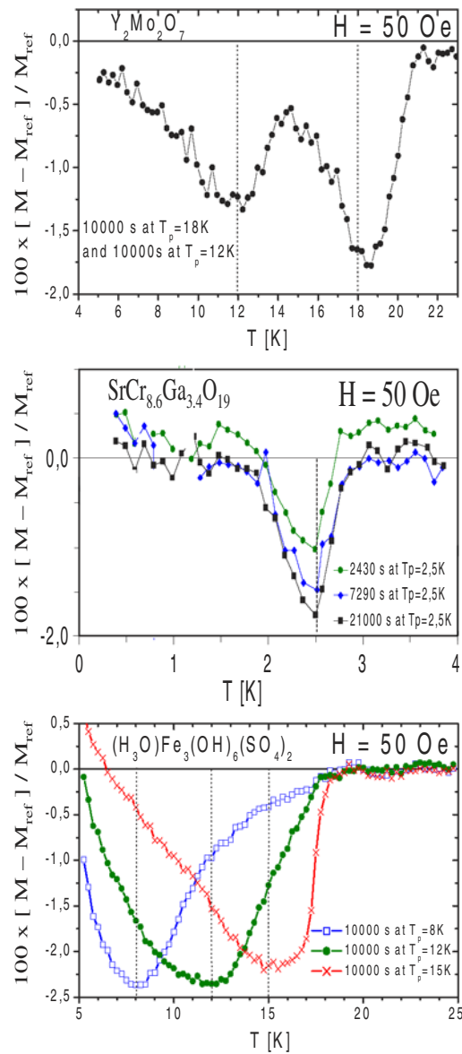
Figure 2. Memory dip experiment (see text): M_{\text{ref}} is measured in a standard ZFC experiment, while M(T) corresponds to the experiment where the cooling was interrupted for a time t_w at a temperature T_p (marked by the dotted lines). From top to bottom: YMO, SCGO, Kagomé samples. The width of the memory dip is quite small in YMO and in SCGO (just as in standard spin glasses). It turns out to be much larger in the Kagomé sample.
