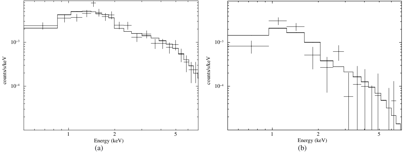
Fig. 4. ACIS-S spectra for the putative pulsar (a) left and entire PWN (b) right . The solid lines correspond to the respective best-fit spectral models. The plots have been rebinned for visual clarity.
