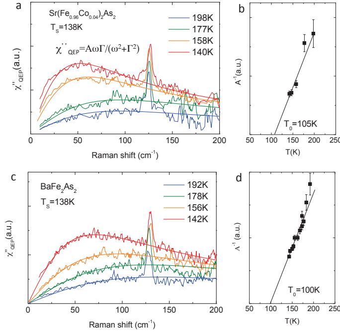
Fig. 3. (Color online). a,c: Temperature dependence of the extracted quasi-elastic peak (QEP) contribution for BaFe 2 As 2 and Sr(Fe 0.96 Co 0.04 ) 2 As 2 along with fits using a relaxational Lorentzian form (see text). b, d: temperature dependences of the inverse of the divergent contribution to the static charge nematic susceptibility, A^{-1} , extracted from the Lorentzian fits. The lines are linear (Curie-Weiss) extrapolation of the data between 200 K and T_S=138 K, allowing a determination of the characteristic temperature T_0 for both systems.
