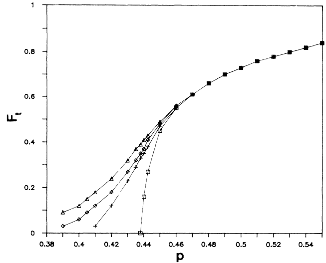
FIG. 12. Mean turbulent fraction F_t as a function of the probability p for different \bar{p} (see text). Squares, \bar{p}=0 ; crosses, \bar{p}=5 \times 10^{-4} ; diamonds, \bar{p}=10^{-3} ; triangles, \bar{p}=2 \times 10^{-3} .
