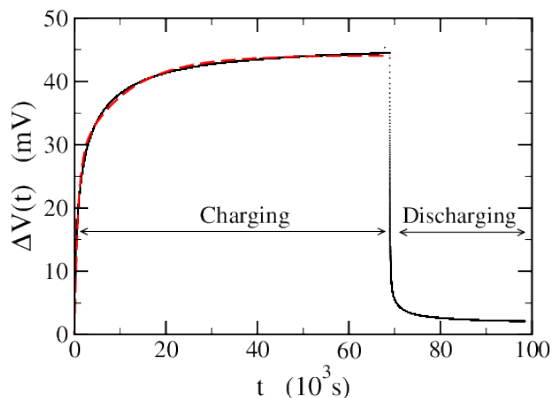
FIG. 4. Charge/discharge potential of the TCC with Pt foil electrodes as a function of time. At time t = 0 , the TCC is completely discharged and charging potential is measured in open circuit (cell connected to the electrometer alone) during 19 hours up to a steady-state value. Discharged is then accomplished by connecting the electrodes to a 20\text{ M}\Omega resistor. During the whole process the top and bottom electrode are maintained at 50^\circ\text{C} and 30^\circ\text{C} respectively. The dashed red line is fit to a sum of two exponentials with characteristic times \alpha = 790\text{ s} and \theta = 10600\text{ s} .
