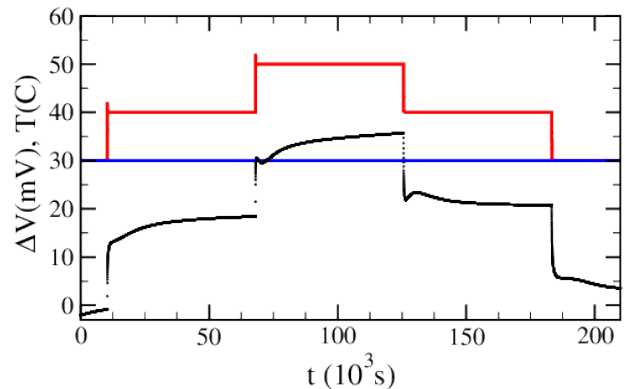
FIG. 2. Thermoelectric potential \Delta V (black line) for a solution of EMIMTFSI (2M) in acetonitrile when the temperature of the top electrode (red line) is changed by a 10 °C step between 30°C and 50°C. The temperature of the bottom electrode (blue line) is maintained at 30°C.
