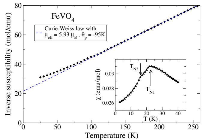
Fig. 2. Thermal variation of the inverse susceptibility in \text{FeVO}_4 ; the inset shows the low temperature variation of the susceptibility.
