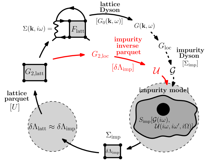
FIG. 5. The QUADRILEX loop. The parts in black correspond to the DGA in the parquet version [the dashed line shows how DGA proposes to update the Weiss field \mathcal{G}(i\omega) ]. The parts in red correspond to the additional steps necessary to update the bare impurity vertex \mathcal{U}(i\omega, i\omega', i\Omega) . For \Sigma we show only the terms beyond Hartree-Fock. The terms in square brackets denote the fixed terms in the solution of the Dyson/parquet equations.
