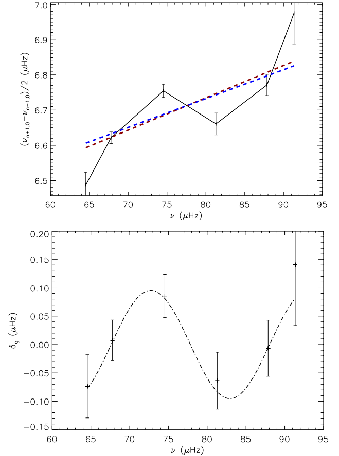
Fig. 2. Top: variation of the large separation as a function of frequency for the star KIC1872166. Error bars correspond to the 1\sigma uncertainties. The general trend is due to the second-order term (the curvature) and the modulation is due to the presence of acoustic glitches. The red dashed line is a linear fit over the oscillations to estimate the curvature parameter. The blue dashed line is the value of the mean curvature given by Mosser et al. (2013) Bottom: variation of the large separation \delta_n as a function of frequency after suppressing the curvature term. The dotted-dashed line shows a fit obtained for this star using Eq. (8).
