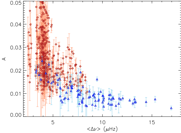
Fig. 5. Dimensionless amplitude \mathcal{A} of the modulation measured as a function of the large separation. Clump stars are indicated by red diamonds and RGB stars by blue triangles. Error bars correspond to the 1\sigma uncertainties.
