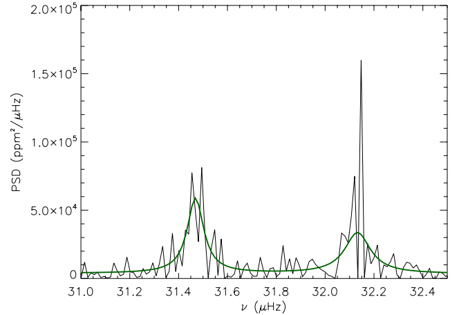
Fig. 1. Power density spectrum (PSD) of the red clump star KIC2303367. The peak around 32.1 \mu\text{Hz} is a radial mode and the peak on the left is the nearby \ell = 2 mode. The Lorentzian fits are shown with the solid green line.
