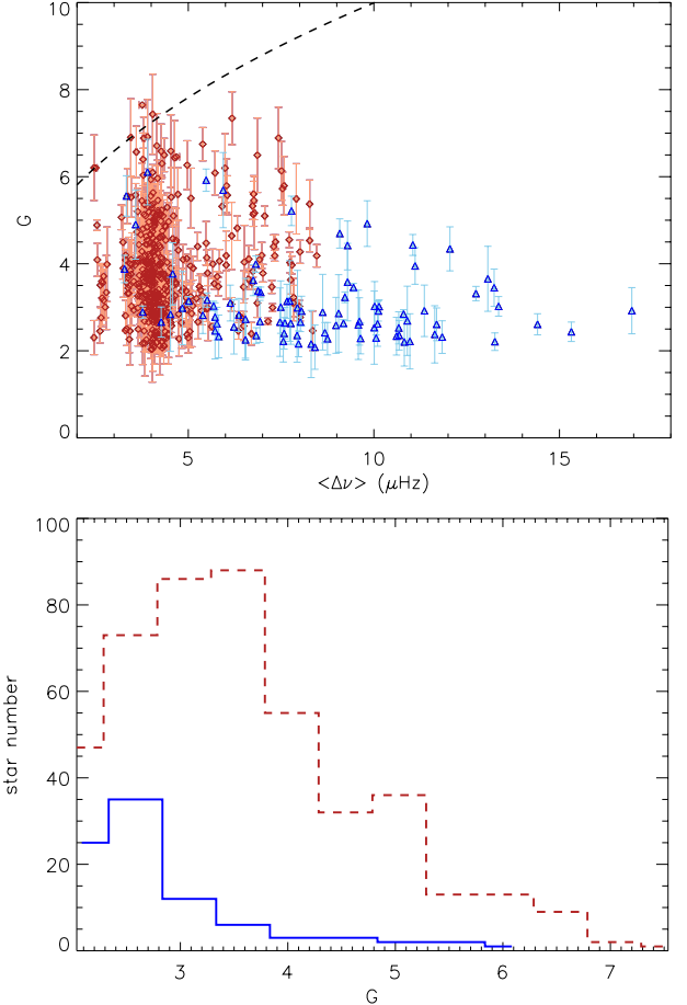
Fig. 4. Top: dimensionless period \mathcal{G} of the modulation measured as a function of the large separation. Clump stars are indicated by red diamonds and RGB stars by blue triangles. Error bars correspond to the 1\sigma uncertainties. The dashed black line indicates the maximum number of radial modes observable in a red giant spectrum. Bottom: histogram of the dimensionless period \mathcal{G} . Clump stars are indicated by the red dashed line and RGB stars by the blue line.
