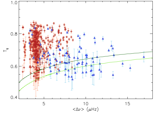
Fig. 7. Acoustic radius of the discontinuity related to the second helium ionization zone as a function of the global large separation. Clump stars are indicated by red diamonds and RGB stars by blue triangles. Error bars correspond to the 1\sigma uncertainties. The light green line indicates the theoretical acoustic radius of the second helium ionization zone for a 1 M_{\odot} star during the RGB phase. The dark green line gives the same information for a 1.4 M_{\odot} star.
