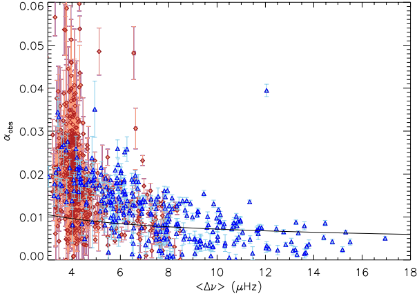
Fig. 3. Apparent curvature \alpha_{\text{obs}} as a function of the large separation for each red giant stars. Clump stars are indicated by red diamonds and RGB stars by blue triangles. Error bars correspond to the 1\sigma uncertainties. The solid black line correspond to the value of the mean curvature \alpha found by Mosser et al. (2013).
