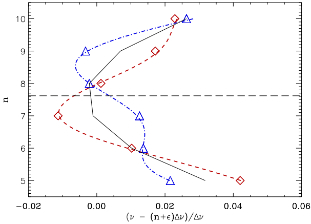
Fig. 9. Synthetic échelle diagram of the radial modes of a typical red giant star with a large separation of 3.90 \mu\text{Hz} . The glitch contributions are overplotted with a dashed red line and red diamonds for a typical clump star, and with a dot-dashed blue line and blue triangles for a typical RGB star. The horizontal dashed black line with a n value of approximately 7.6 represents the n_{\text{max}} value. Only six radial modes are shown in this figure, which is typically the number of observed modes.
