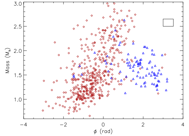
Fig. 8. Stellar masses in function of the phase of the modulation. Clump stars are indicated by red diamonds and RGB stars by blue triangles. The black box in the right corner of the figure corresponds to the typical 1\sigma uncertainties for these parameters.
