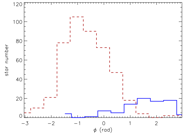
Fig. 6. Top: phase \phi of the modulation measured as a function of the global large separation. Clump stars are indicated by red diamonds and RGB stars by blue triangles. Error bars correspond to the 1\sigma uncertainties. Bottom: histogram of the phase \phi . Clump stars are indicated by the red dashed line and RGB stars by the blue line.
