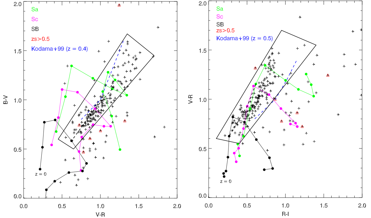
Fig. 2. B - V vs. V - R (left) and V - R vs. R - I (right) diagnostic diagrams. The sample, comprising 202 unique objects with counterparts in the M05 catalogue is denoted by crosses (+). The red triangles ( \Delta ) denote objects with spectroscopic redshift z_s > 0.5 in the M05 catalogue. The control grid has been built using synthetic colours from COSMOS templates for Sa, Sc, and SB galaxies in the range z = 0.0 – 1.0 with steps of \Delta z = 0.1 . The thick black dashed line connects the three templates at z = 0.4 . The blue dashed line depicts the Kodama et al. (1999) models at z = 0.4 and z = 0.5 . The thick black solid line box marks the approximate region used for selecting the cluster candidates.
