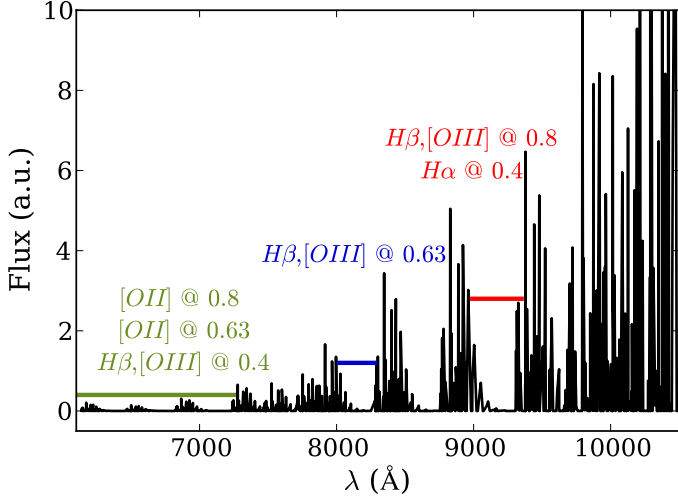
Fig. 1. Night sky spectrum from Rousselot et al. (2000) and GLACE windows within the OH bands. The loci of the strongest rest-frame emission lines at different redshifts are shown next to the corresponding spectral windows. The observations within this paper have been performed within the H \alpha window at z = 0.4 .
