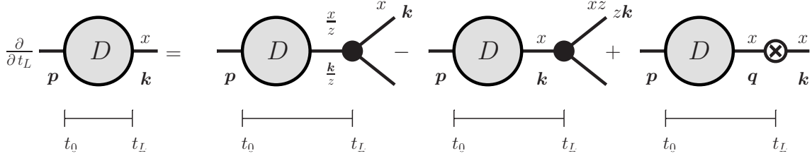
Figure 2. Diagrammatic representation of the forward evolution for the inclusive gluon distribution.
