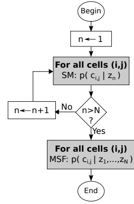
Fig. 2. Overview of Occupancy Grid Algorithm
