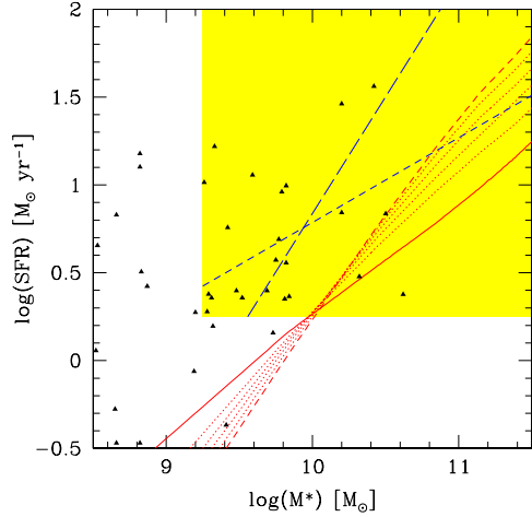
Fig. 5. Stellar mass-SFR relation of LGRB hosts (symbols) compared to that taken from the models of Boissier et al. (2010) for SFGs shown as a set of curves (solid at redshift 0, dashed at redshift 1.1, dotted for intermediate redshifts). The shaded area corresponds to our completeness limits. The dashed lines within this area are the two regression lines (for the SFR as a function of the stellar mass and the stellar mass as a function of the SFR) computed from the LGRB hosts data.
