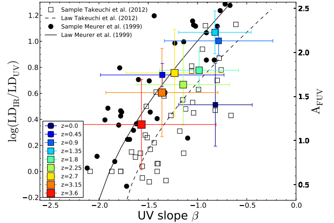
Fig. 3. Dust attenuation vs. redshift. Note that the x -axis bars correspond to the dispersion in UV slope while the y -axis bars are evaluated from the uncertainties in the LFs. The black dots denote the original data points from Meurer et al. (1999) and the black curve plots the law of Meurer et al. (1999). The black dashed line and gray boxes denote the update (using the same apertures in FUV and in FIR) from Takeuchi et al. (2012). Strictly speaking, our points and those from Meurer et al. (1999) are not comparable because we used volume-corrected LFs and not individual galaxies as in Meurer et al. (1999). In the diagram, the color-coded points show an almost continuous decrease with increasing redshift and lie in between the Meurer et al. (1999) and Takeuchi et al. (2012) laws. We emphasize that the dust attenuation A_{\text{FUV}} is estimated from the IRX and not from the UV slope \beta .
