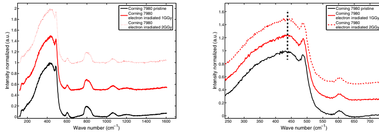
Fig. 3. (Left) Raman spectra normalized at the highest peak of pristine and electron irradiated samples at 1 and 2 GGy ( \lambda=532 nm). (Right) Raman spectra normalized and zoomed ( 250-700\text{cm}^{-1} ) in on the highest peak for pristine and 1 and 2 GGy electron irradiated samples ( \lambda=532 nm).
