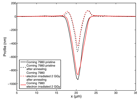
Fig. 6. AFM profiles of indentation on pristine (black line) and irradiated samples at 2 GGy (red line) before (solid line) and after annealing (dotted line) The indentation load is 50 g, and the profiles are parallel to the edges of indentation. These profiles are the mean profiles of 5 profiles extracted from 5 indentations
