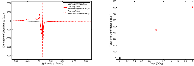
Fig. 2. (Left) EPR spectra of Corning 7980® pristine and electron irradiated at 1 and 2 GGy ( P=10 mW, f=9.82 GHz). (Right) Total amount of defects created in \text{a-SiO}_2 at different integrated doses .
