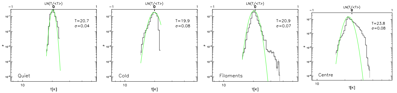
Fig. 6. Same as Fig. 5 for temperature. The x-axis labelling for the temperature PDF is in Kelvin at the bottom x-axis and in \ln(T/\langle T \rangle) at the top x-axis. The width, \sigma , and the peak temperature, in Kelvin, of the PDF are given in each panel.
