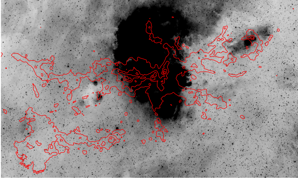
Fig. A.1. H\alpha image of NGC 6334 ( 2.2 \times 1.3 ). The isocontours represent the Herschel -500 \mu\text{m} intensity (the five contours levels are from 6 Jy/beam to 656 Jy/beam in equal logarithmic steps).
