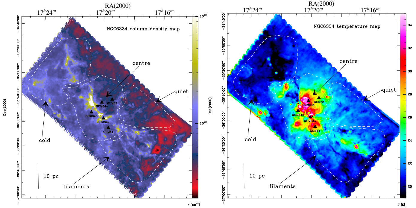
Fig. 3. H_2 column density (left) and temperature (right) maps of NGC 6334, determined using the 160 \mu m , 250 \mu m , 350 \mu m , and 500 \mu m Herschel wavebands. The different sub-regions discussed in the text are indicated with white dashed-line polygons. The H II regions GUM61 to 64a,b,c are indicated with triangles.
