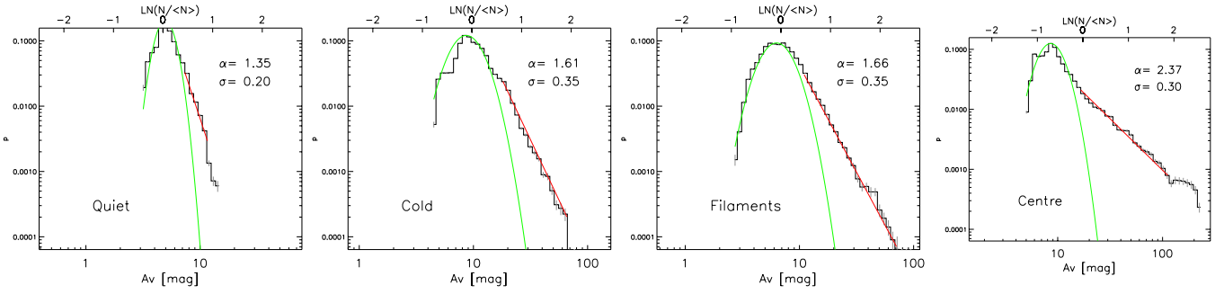
Fig. 5. Column density PDFs of the 4 sub-regions in NGC 6334 produced without the 70 \mu\text{m} band. The x-axis labelling is in visual extinction at the bottom x-axis and in \ln(N/\langle N \rangle) at the top x-axis. The labelling of the y-axis is a probability. The green curves indicate the best lognormal fit PDF (Eq. (1)), and the red line is a fit to the high-density part of the PDF that follows a power law. The width of the PDF, \sigma , and the exponent of the spherical density profile, \alpha , are given in each panel.
