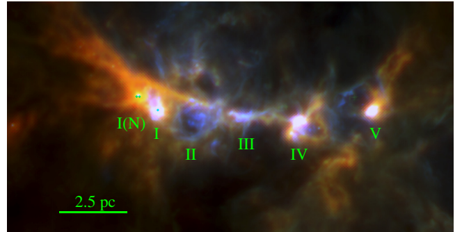
Fig. 2. Three-colour image of the central part of NGC 6334 with the same colour mapping as in Fig. 1. The image is 33'.2 \times 17'.1 in size and is centred at 17^{\text{h}}20^{\text{m}}35^{\text{s}}.05 , -35^{\circ}49'13''.5 . The higher contrast better highlights active regions of star formation compared to Fig. 1. The nomenclature of the far-infrared sources is from McBreen et al. (1979) and Gezari (1982).
