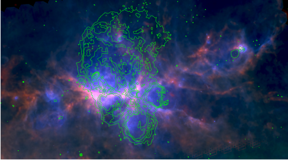
Fig. A.2. Three-colour image ( 1.8 \times 1.0 ) of NGC 6334 with 500 \mu\text{m} data in red, 160 \mu\text{m} data in green, and 70 \mu\text{m} data in blue. The H\alpha isocontours are overlaid (the five contours levels are, in arbitrary units, from 6000 to 15 000 on a linear scale).
