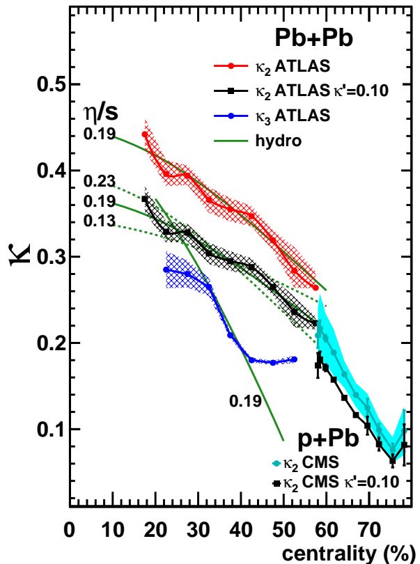
FIG. 2. (Color online) Response coefficients \kappa_2 and \kappa_3 versus centrality. Symbols: results from the fits to ATLAS Pb+Pb data [10] and to CMS p+Pb data [11]. For \kappa_2 , systematic and statistical experimental errors are added in quadrature. For \kappa_3 , only the statistical error is shown. Also shown are \kappa_2 values from fitting the v_2 distributions with a non-linear term characterized in Eqs. (10 and 11) by \kappa' . The smooth solid lines are the result of a viscous hydrodynamic calculation for \kappa with \eta/s = 0.19 . The upper solid line is normalized up by the factor 1.7, the middle line by the factor 1.4, and the lower line ( \kappa_3 ) by the factor 3.2. The dashed lines for \kappa_2 with \kappa' = 0.1 are shown for comparison: they are for hydro results with \eta/s = 0.13 (normalized up by 1.2) and \eta/s = 0.23 (normalized up by 1.6).
