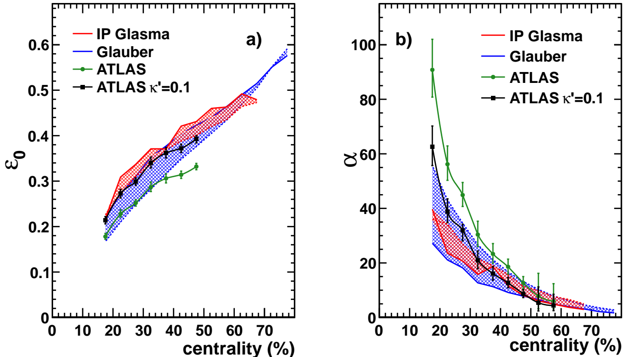
FIG. 3. (Color online) \varepsilon_0 (a) and \alpha (b) versus centrality. Symbols: results from the fits to ATLAS v_2 data. Predictions from the Monte-Carlo Glauber [28] and IP-Glasma [29, 30] models are shown as shaded bands. Also shown are values from fits with a non-linear term defined by \kappa' in Eq. (10).
