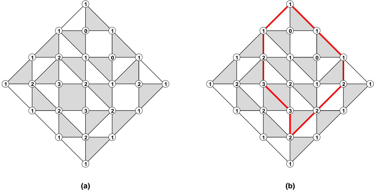
FIGURE 2. The tessellated shadow of the point (i, j, 4) onto a particular initial data stepped surface. We have indicated for each vertex (x, y) \in \mathbb{Z}^2 of the (i, j) plane projection the corresponding value of k = k_{x,y} in a circle. The center is at coordinates (i, j, 2) .
