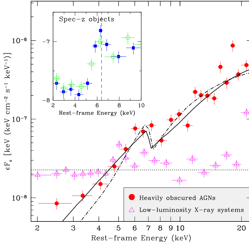
FIG. 5.— Flux density versus rest-frame energy showing the composite rest-frame 2–20 keV spectra for the heavily obscured AGNs (filled circles; all objects except the X-ray bright AGN J033222.5–274603) and low-luminosity X-ray systems (open triangles) as compared to an unabsorbed power-law model (dotted line; \Gamma = 2.0 ), a pure reflection model (solid curve; \Gamma = 1.7 ), and the best-fitting model to the reflection-dominated z \approx 0 AGN Swift J0601.9–8636 (dot-dashed curve; Ueda et al. 2007); see §3.1.4. The inset panel shows the stacked X-ray spectra at rest-frame 2–10 keV of the heavily obscured AGNs with spectroscopic redshifts (filled squares: all objects; open circles: all objects except J033235.7–274916, which has been individually identified with Fe K \alpha emission; Feruglio et al. 2011); the dashed line shows the expected rest-frame energy of Fe K \alpha . The properties of the heavily obscured AGNs are consistent with those expected for reflection-dominated systems and \approx 10 –50% are likely to be Compton-thick AGNs (see §3.1.4).
