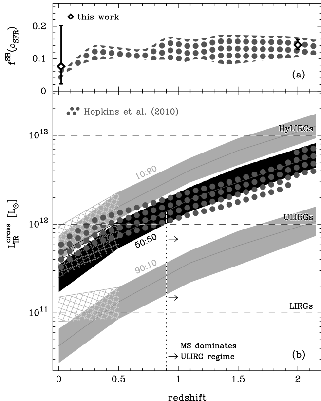
FIG. 4.— (a): Constraints on the fractional contribution f_{\text{SB}}^{\text{SB}}(\rho_{\text{SFR}}) of starbursts to the cosmic SFRD at z = 0 and 2, compared to simulation-based evolutionary predictions in Hopkins et al. (2010) (dotted area). (b): Redshift evolution of the cross-over luminosity for equal contributions of normal and burst-like star formation to IR LFs (black; 68% confidence region highlighted). Light grey curves: luminosities at which main-sequence activity contributes 90% (10%) to the global IR LF. Hatched branches: low-redshift evolution assuming the best-fit f_{\text{SB}}^{\text{SB}}(\rho_{\text{SFR}}, z = 0) = 7.6_{-5.4}^{+12.6}\% of panel (a). Main-sequence star formation dominates the ULIRG regime at z \gtrsim 0.9 (dotted vertical line).
