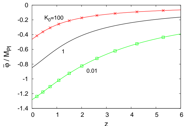
FIG. 5: Normalized scalar field \tilde{\varphi}/M_{\text{Pl}} for the same models as in Fig. 1.
