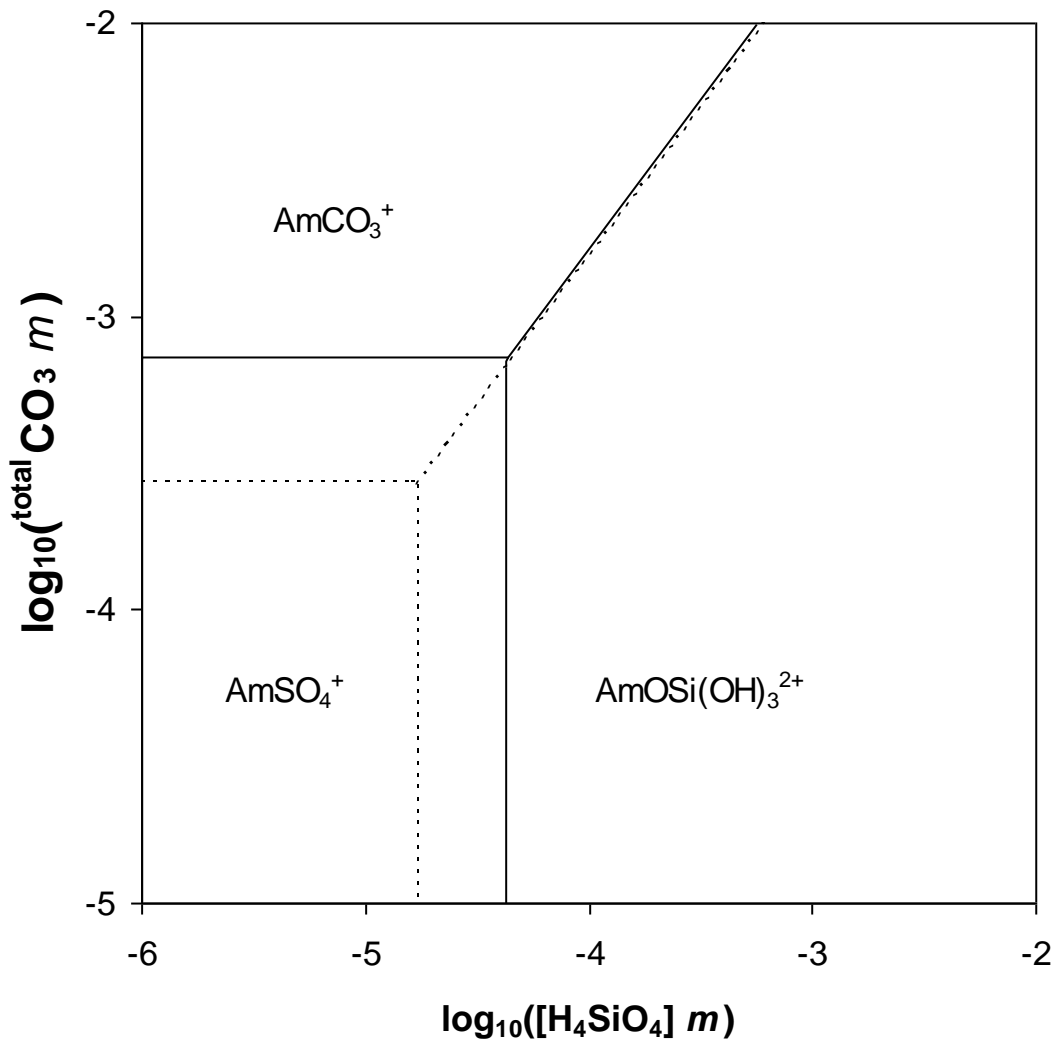
Figure 11. Predominance diagram of traces of americium(III) at pH 7, total sulphate concentration between 14 mM (dotted) and 40 mM (plain), 0.1 mol \text{NaClO}_4 /L, and varying [\text{Si(OH)}_4(\text{aq})] and total carbonate. Thermodynamic data from Guillaumont et al. (2003), except for \text{Am}(\text{SO}_4)_n^{3-2n} from Silva et al. (1995).
