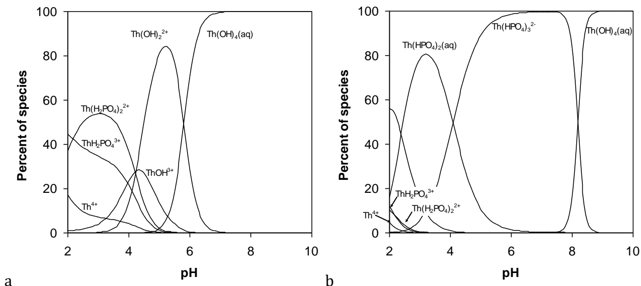
Figure 6 Solution speciation of the thorium phosphate system at I = 0.1 \text{ mol/L (NaClO}_4\text{)} , [\text{PO}_4]_{\text{tot}} = 10^{-4} \text{ mol/L} from the data selected in Rand et al. (2009) (a, left), and including data from Ekberg et al. (2010) in Table 2 (b, right).
